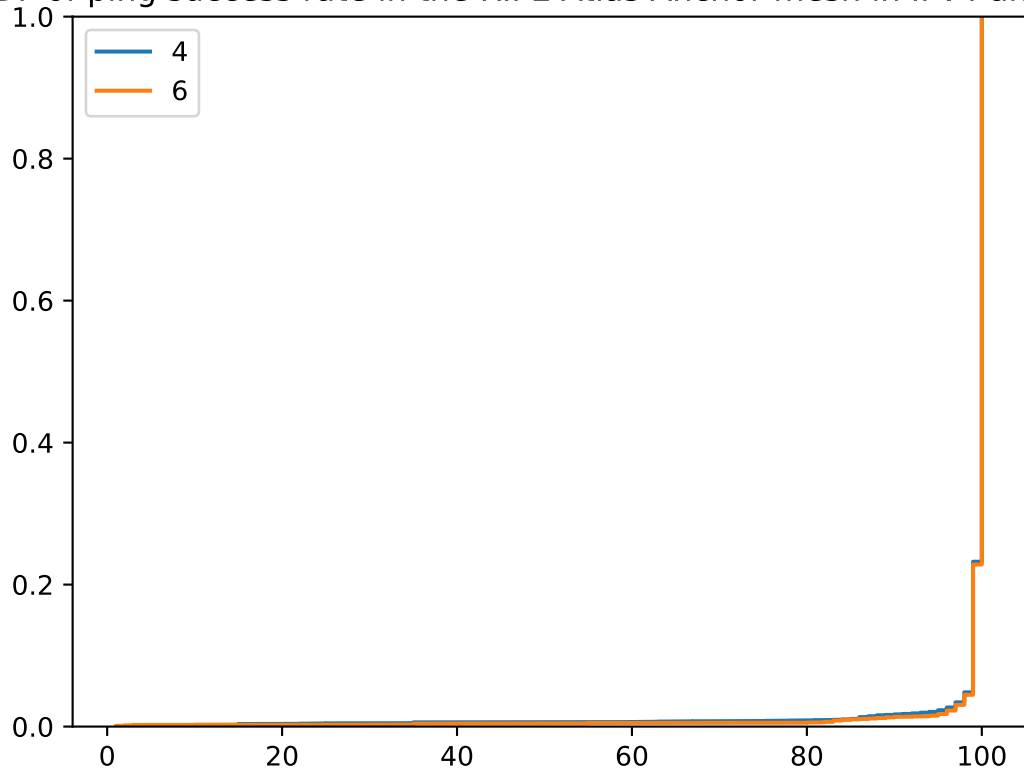
CDF of ping success rate in the RIPE Atlas Anchor mesh in IPv4 and IPv6
