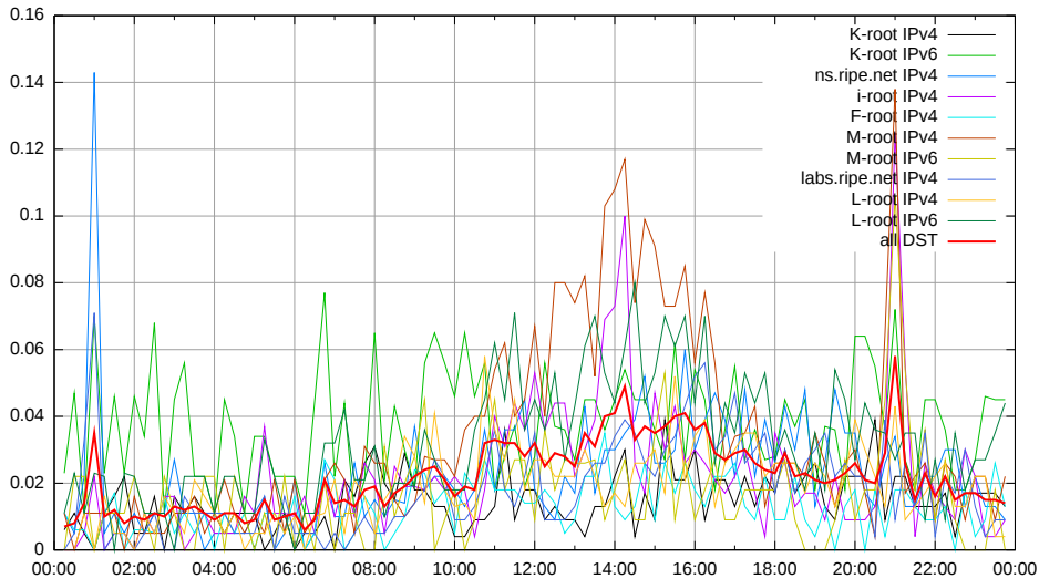
fraction of src/dst-pairs that experienced any pkt loss per 15 min bin, combined (2010-17-17)
