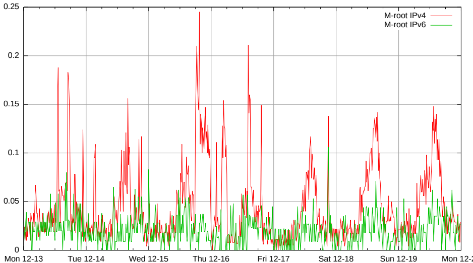
fraction of src/dst-pairs that experienced any pkt loss per 15 min bin: M-root
