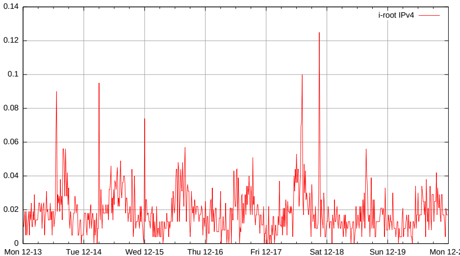
fraction of src/dst-pairs that experienced any pkt loss per 15 min bin: i-root
