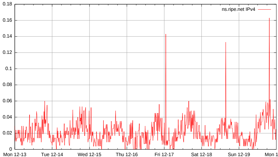
fraction of src/dst-pairs that experienced any pkt loss per 15 min bin: ns.ripe.net
