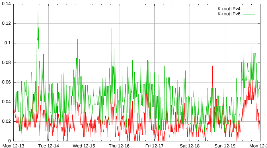
fraction of src/dst-pairs that experienced any pkt loss per 15 min bin: K-root
