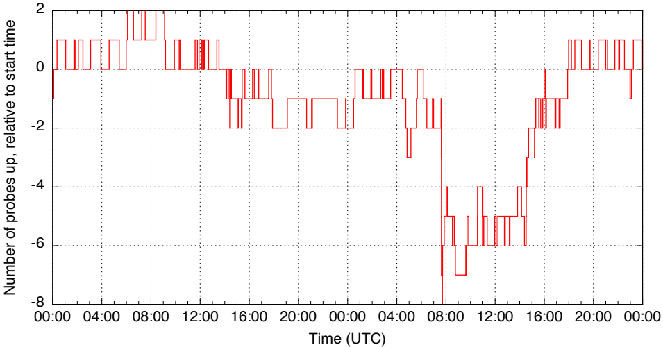
Turkey power outage as seen by RIPE Atlas 2015-03-30 - 2015-03-31
